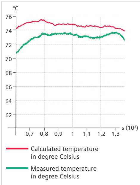
Comparison of stationary oil temperature: simulation vs test.
