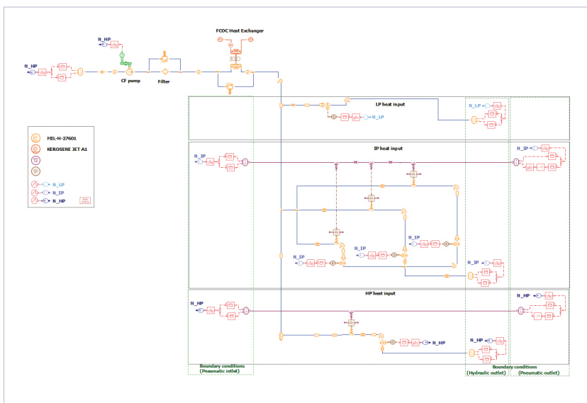
Simcenter Amesim thermal-hydraulic model.
